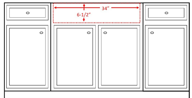
FRONT VIEW OF CABINETS
